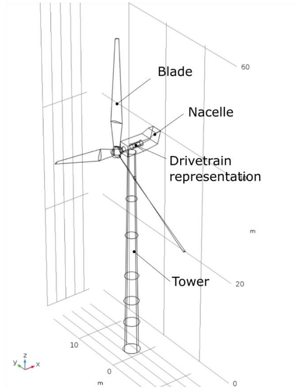
Figure 1. Structural component of the wind turbine with a cylinder representing the drivetrain
